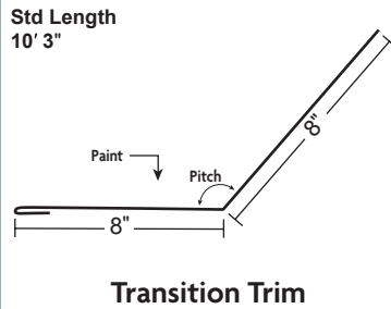
Transition Trim
