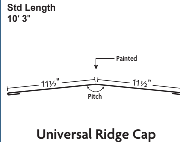
Universal Ridge Cap
