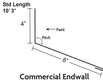
Commercial Endwall
