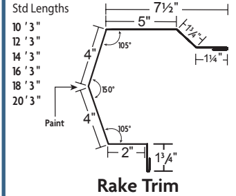
Rake Trim
