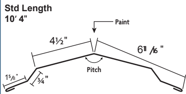
Ridge Cap
