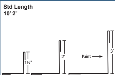
Inside Angle
