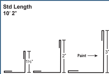
Outside Angle
