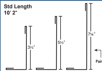
Post Trim
