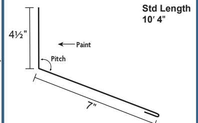
Endwall Trim
