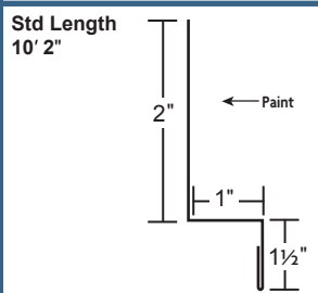
1" Double Angle
