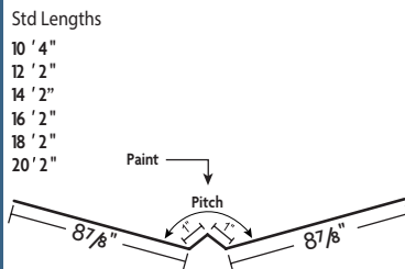
Valley Trim
