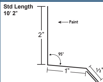
1" Base Trim
