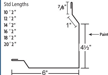
Rake & Corner
