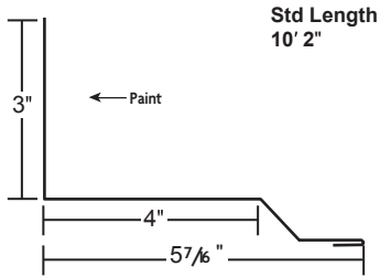
Sidewall Trim
