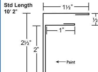
F Channel
