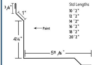
Inside Corner
