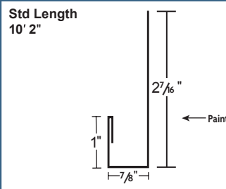
J Trim
